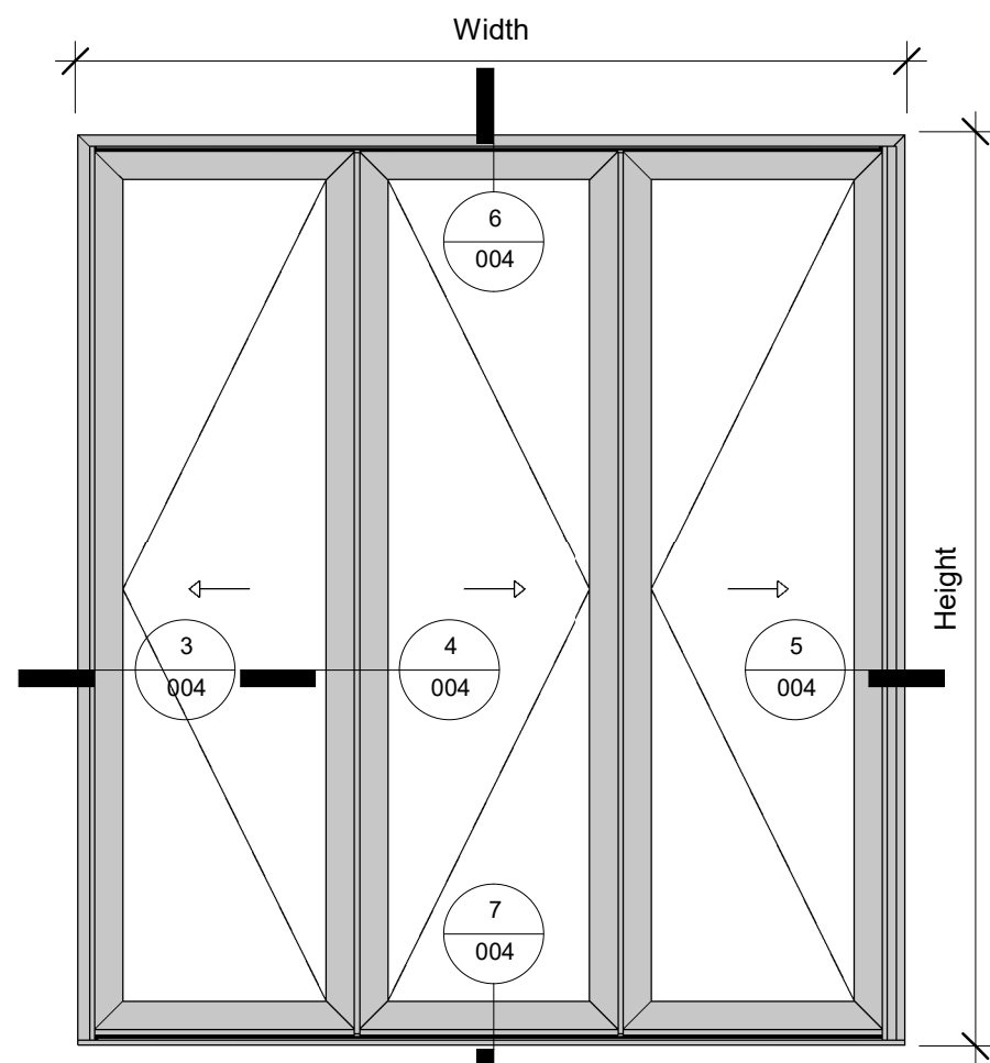
1 Elevation Front 1 : 20
